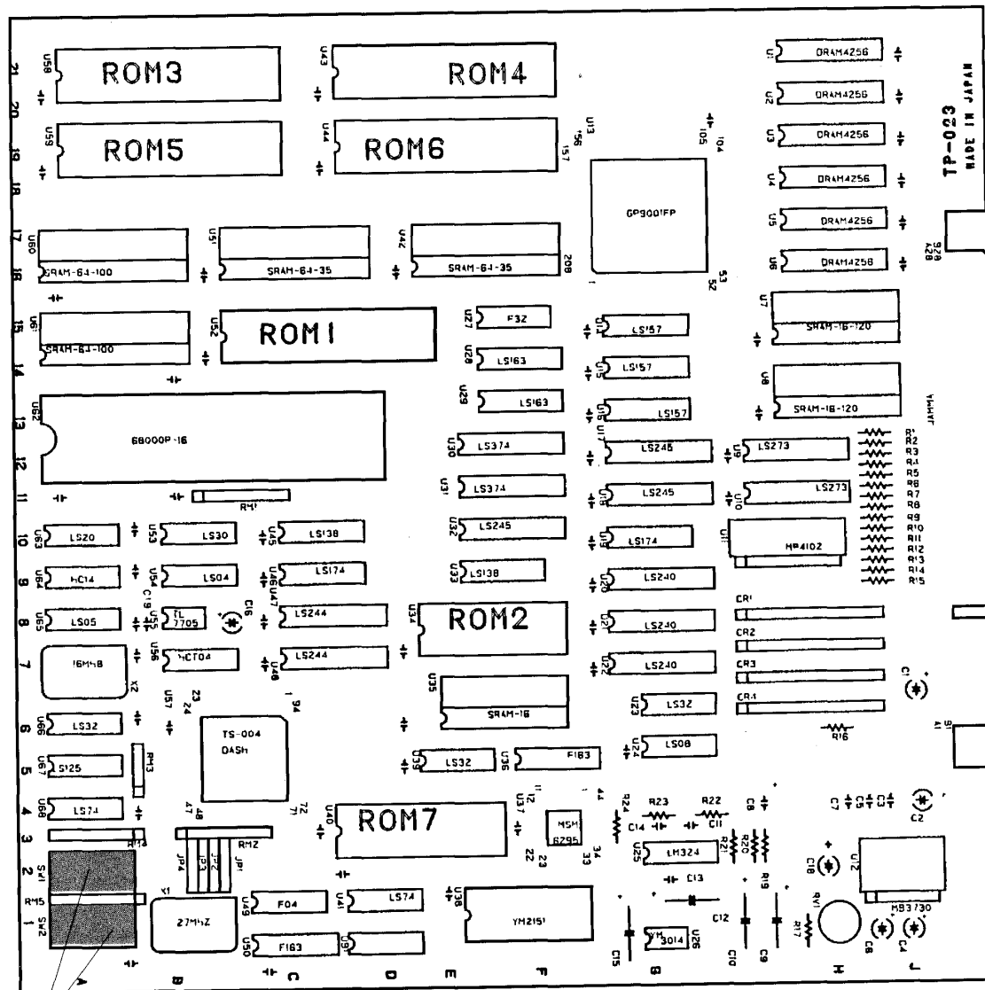
Are both DIP switch locations. Use for setting game and coin options.
